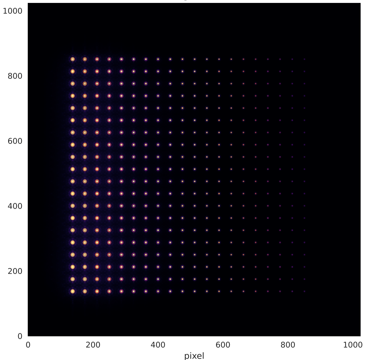
Image Plane
